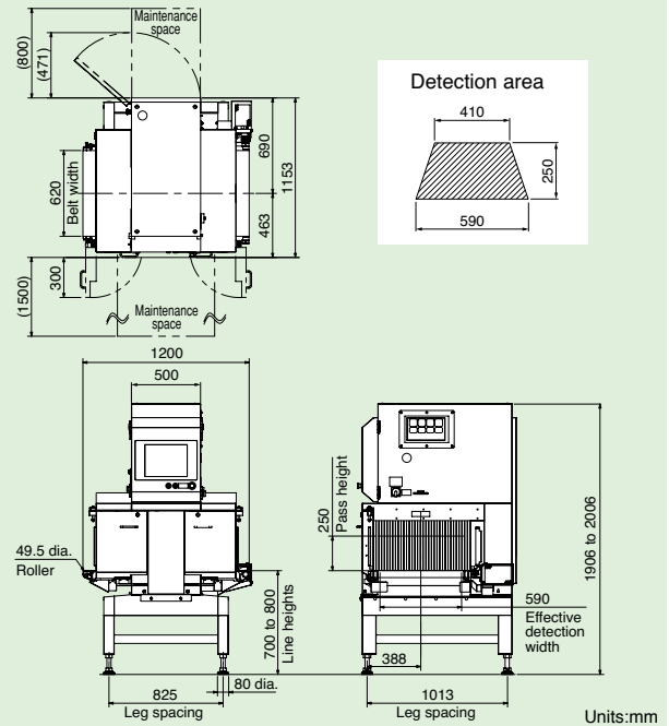
KD7447FWE
